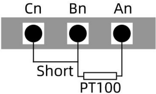
Two-wire connection
