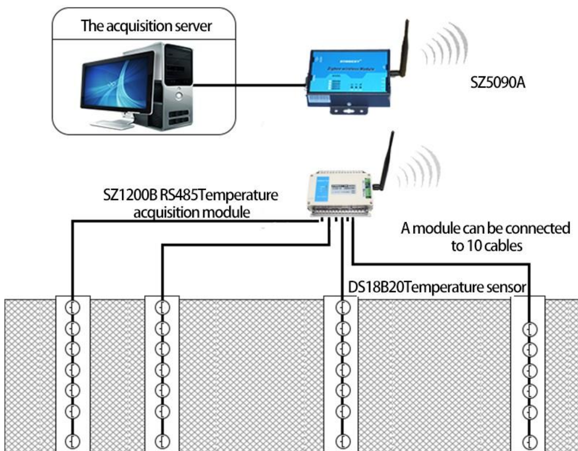
● APPLICATION SCHEME OF TEMPERATURE MEASUREMENT SYSTEM FOR BURIED PIPE
