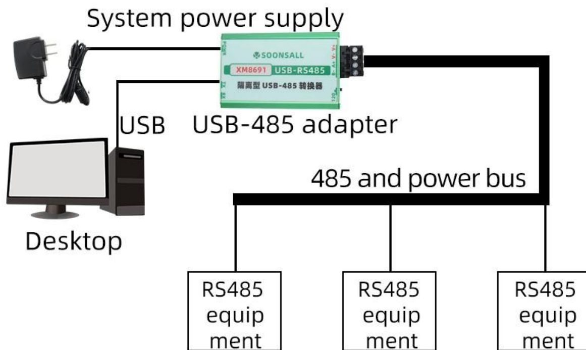
RS485 system shared power scheme
