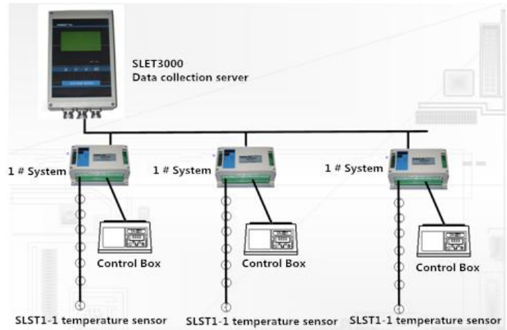
RS485 wireless systems acquisition and control transfer
